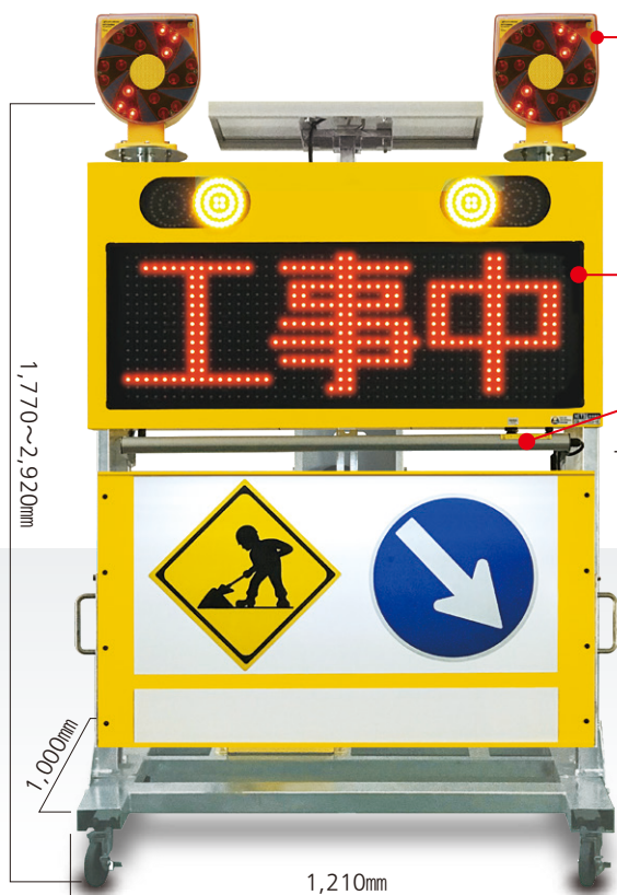
SOC353HS 3面横型(昇降式) 20108
